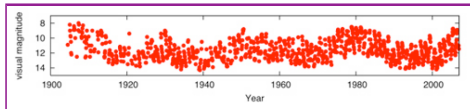
Visual magnitude estimates (25-day averages) of RU Virginis from the AAVSO International Database .
